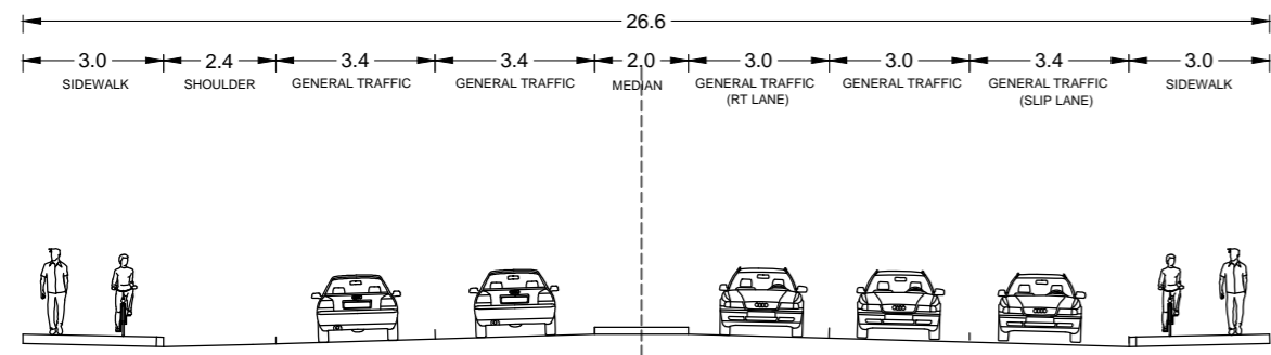
SECTION 1-1
