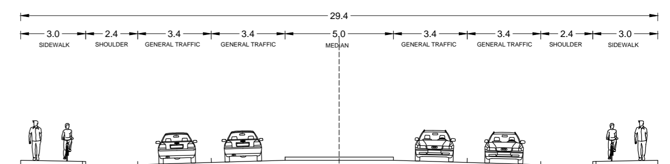
SECTION 3-3
