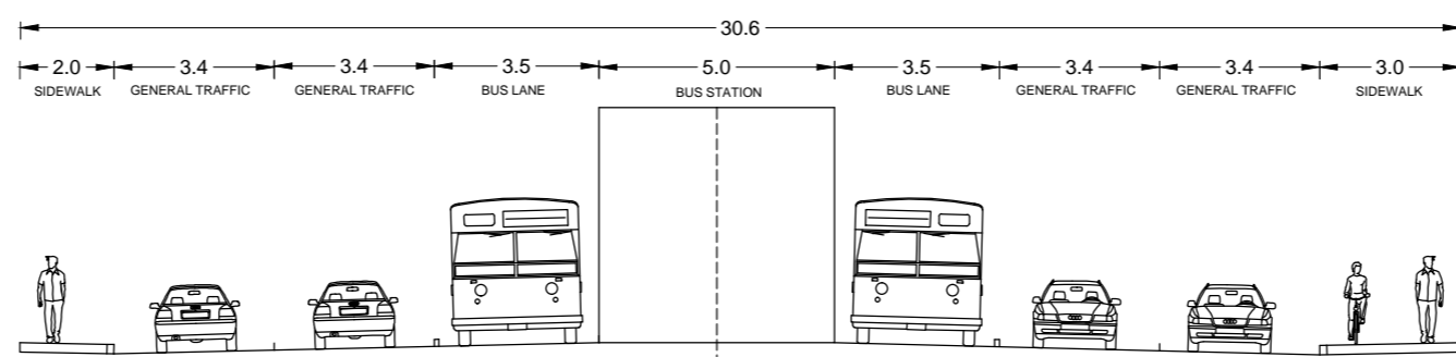
SECTION 2-2
